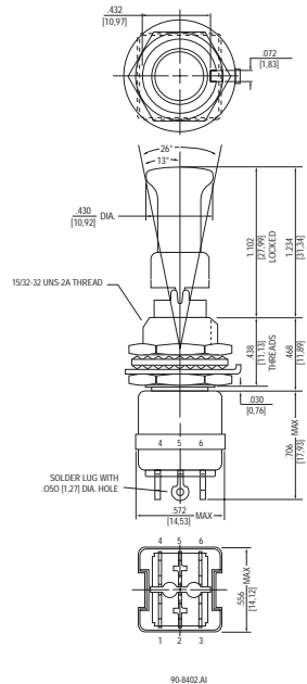
Mushroom Cap Style
