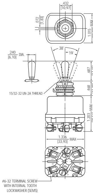
Terminal Identification
