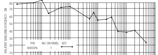
Graphic Illustration defines relative shielding efficiency of RFI shielded component/ components over unshielded device.
