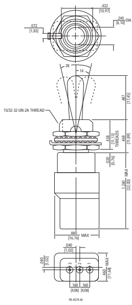
Large Toggle/ Terminal Identification
