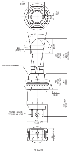
Standard Cap Style
