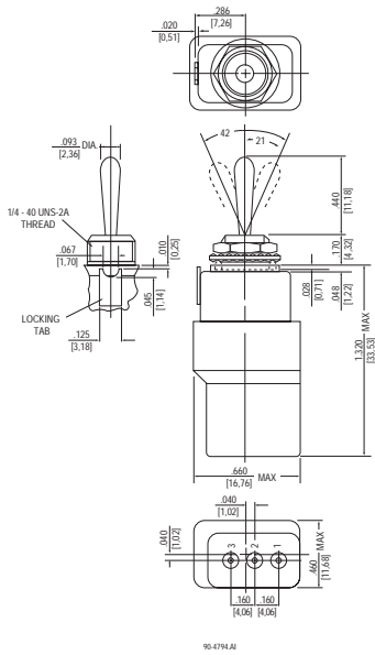
Small Toggle
