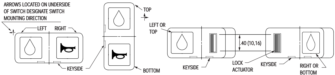
FIGURE 1 Horizontal Mount
