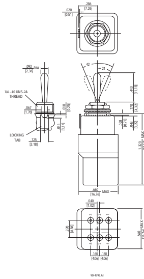
Small Toggle
