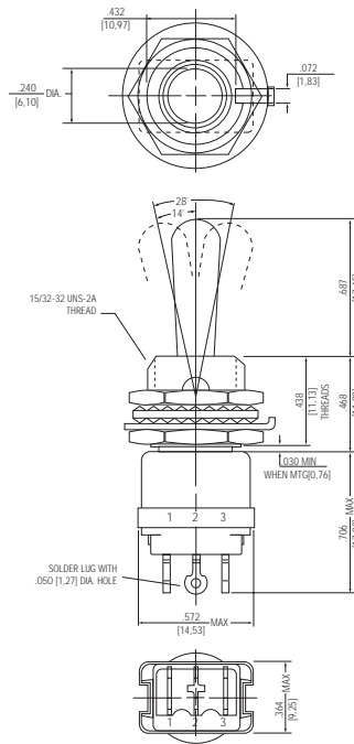
Terminal Identification
