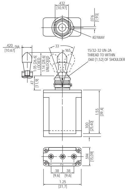
Terminal Identification
