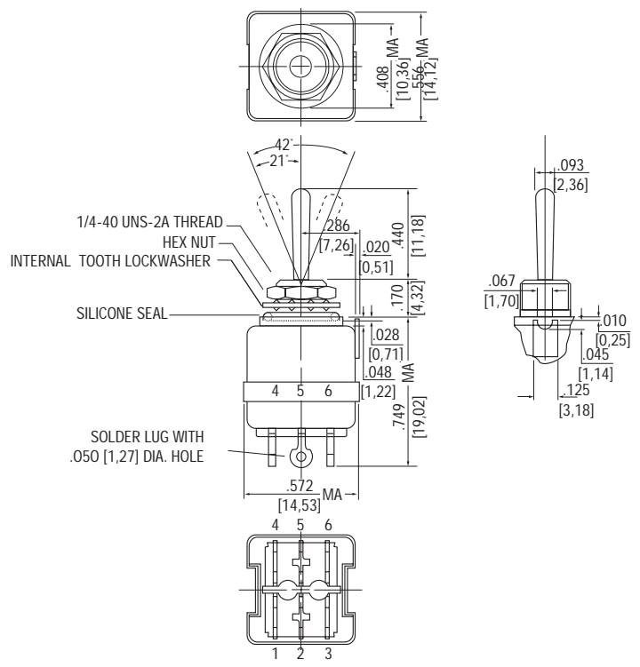
Terminal Identification
