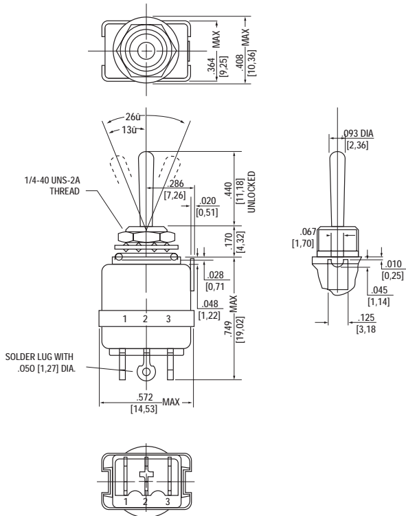
Terminal Identification
