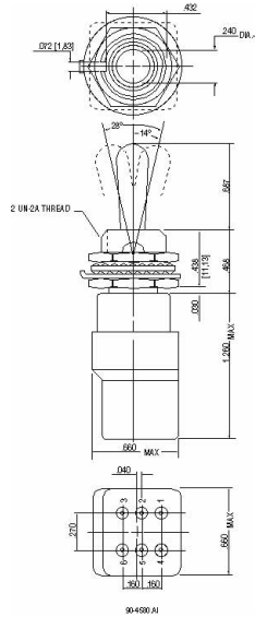
Large Toggle/ Terminal Identification
