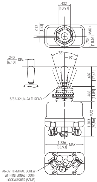
Terminal Identification
