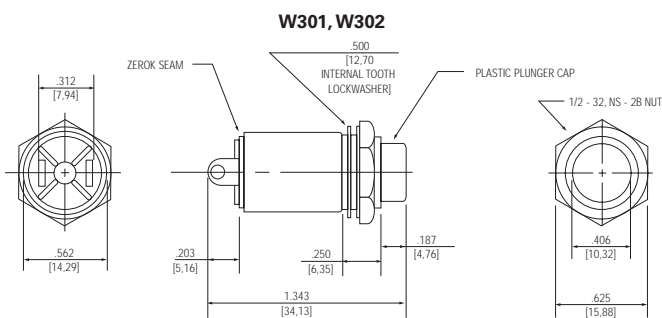
W300 SERIES W/SOLDER TERMINALS
